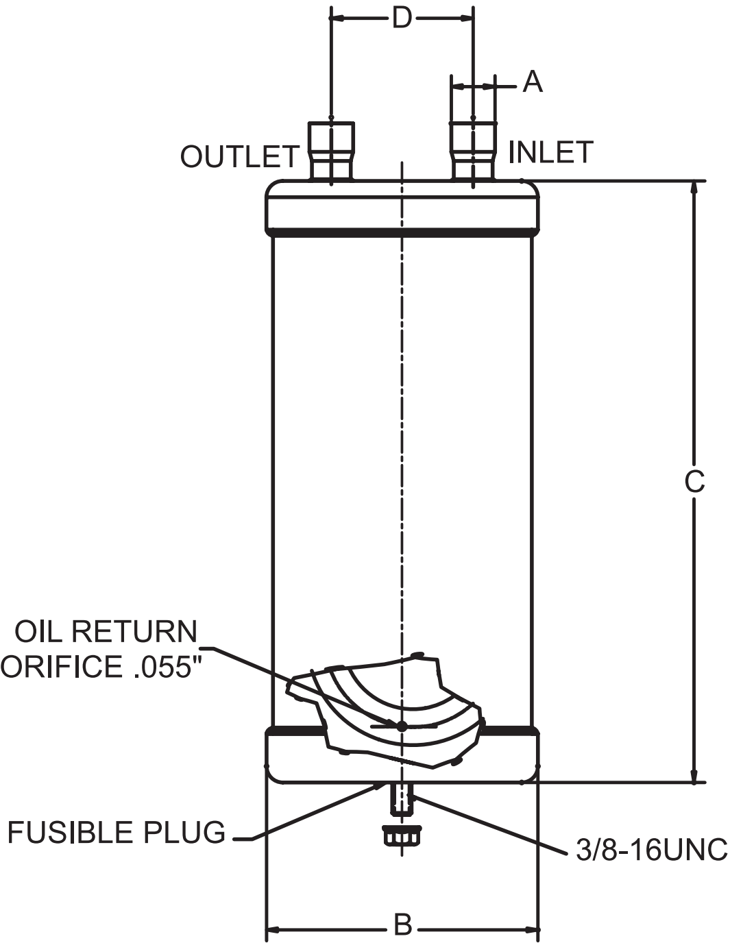
Dimensional data
