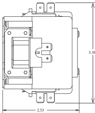
40 AMP MODEL (WITH COVER)
